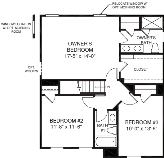
UPPER LEVEL
