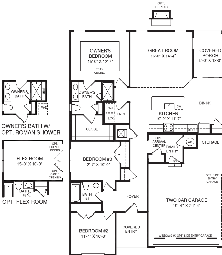
MAIN LEVEL
