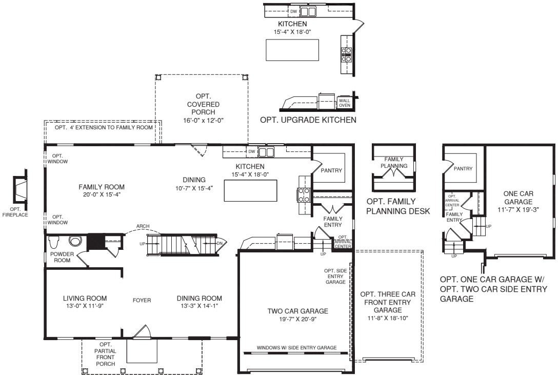
MAIN LEVEL
