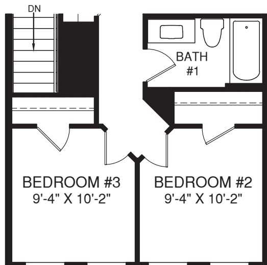
OPT. THIRD BEDROOM W/ ELEV. C ONLY
