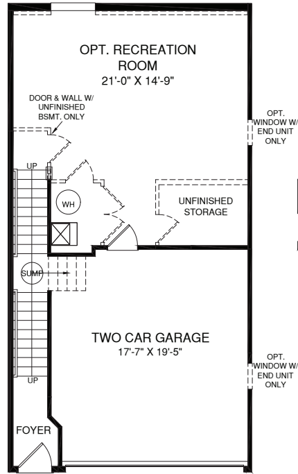
LOWER LEVEL
