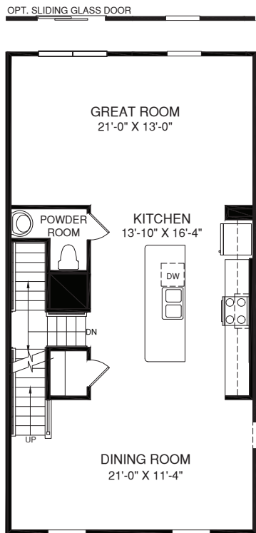
MAIN LEVEL
