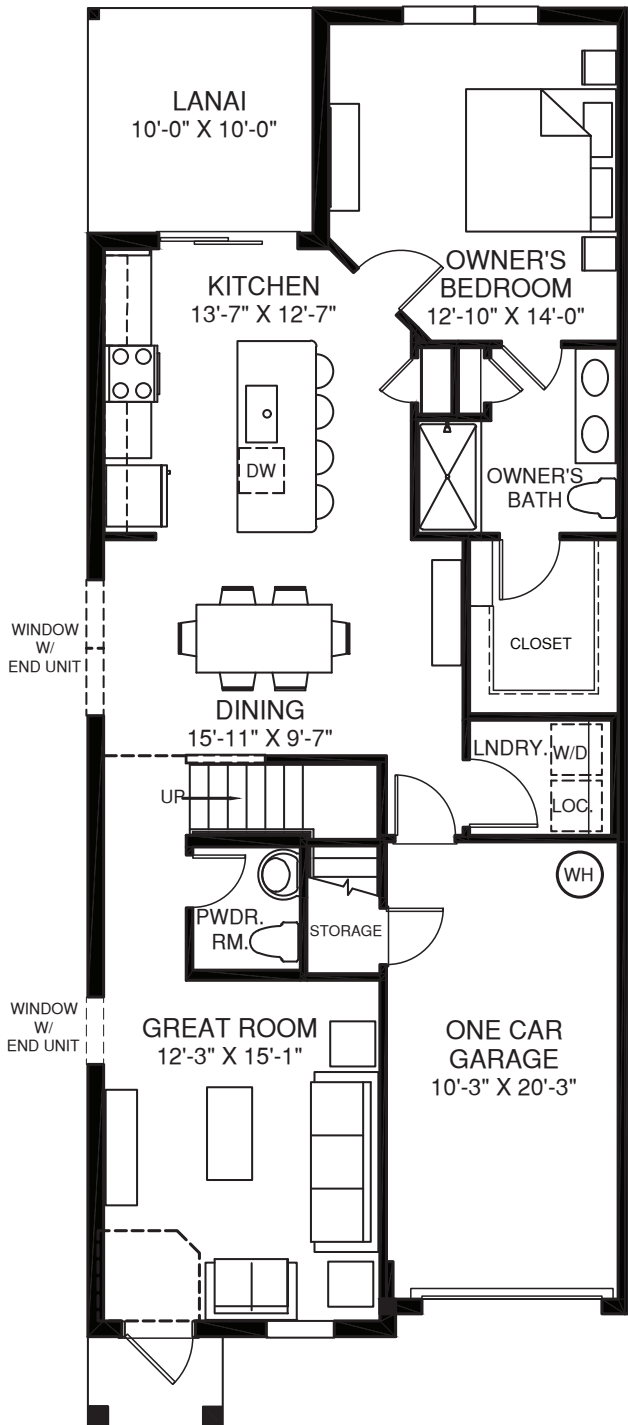
MAIN LEVEL
