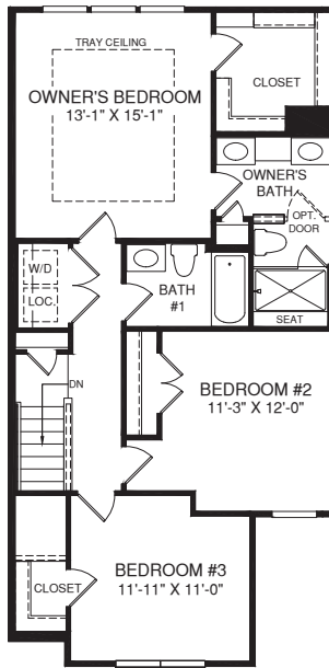
THIRD FLOOR
