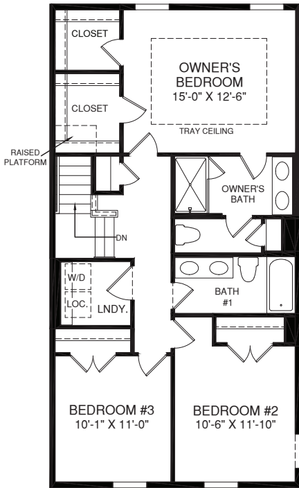
UPPER LEVEL
