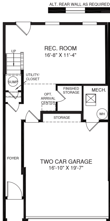
LOWER LEVEL
