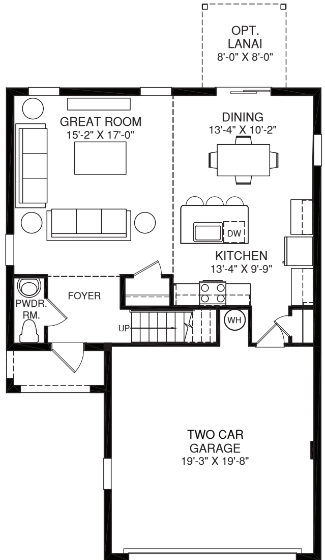
MAIN LEVEL
