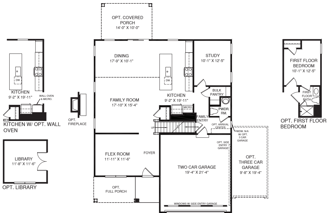
MAIN LEVEL
