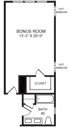
OPT. BONUS ROOM
