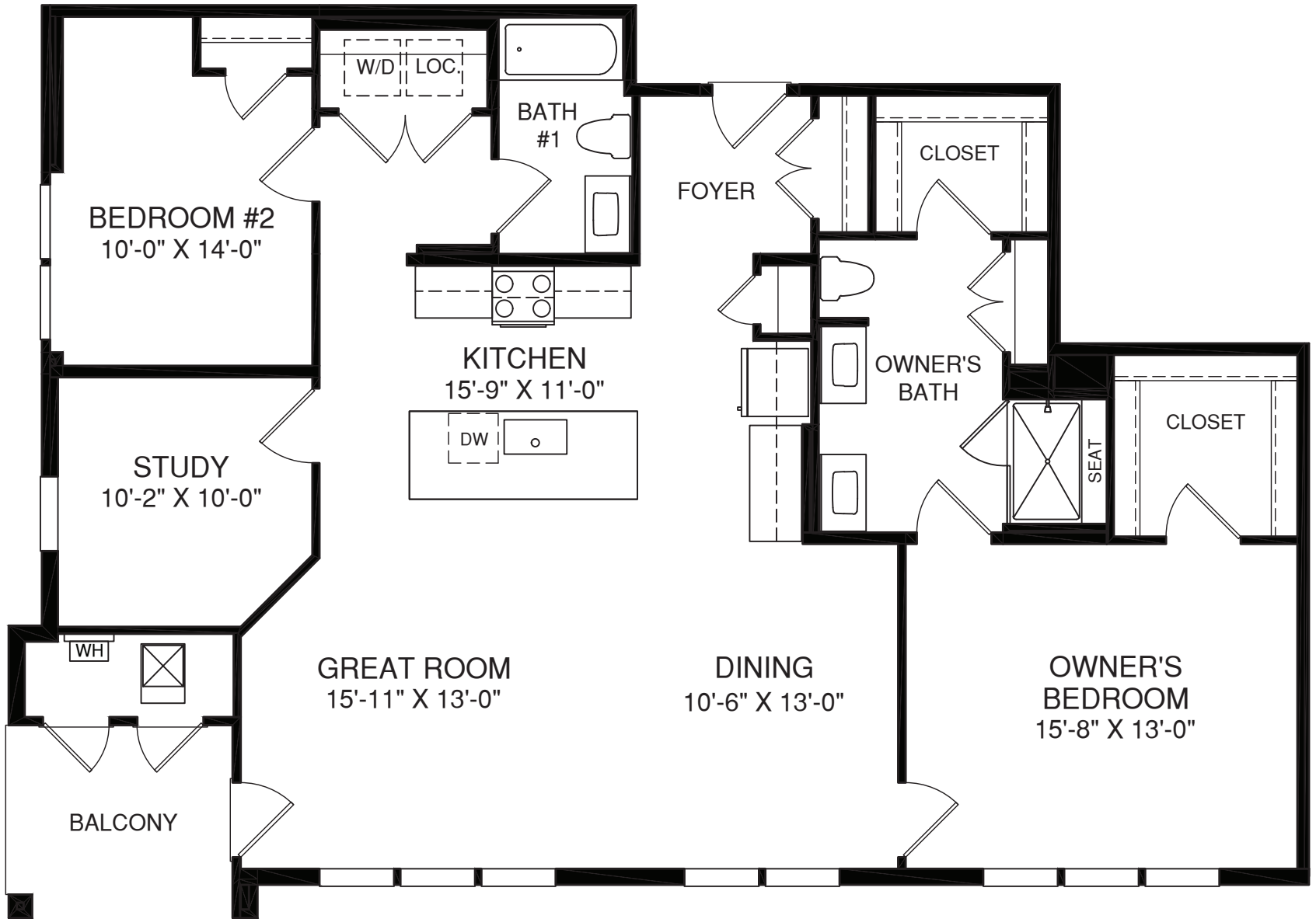
THE SAPPHIRE - LAYOUT 3
