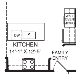
KITCHEN W/ OPT. WALL OVEN
