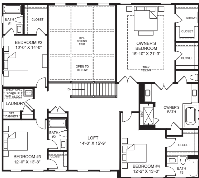
OPT. FOUR BEDROOM W/ LOFT
