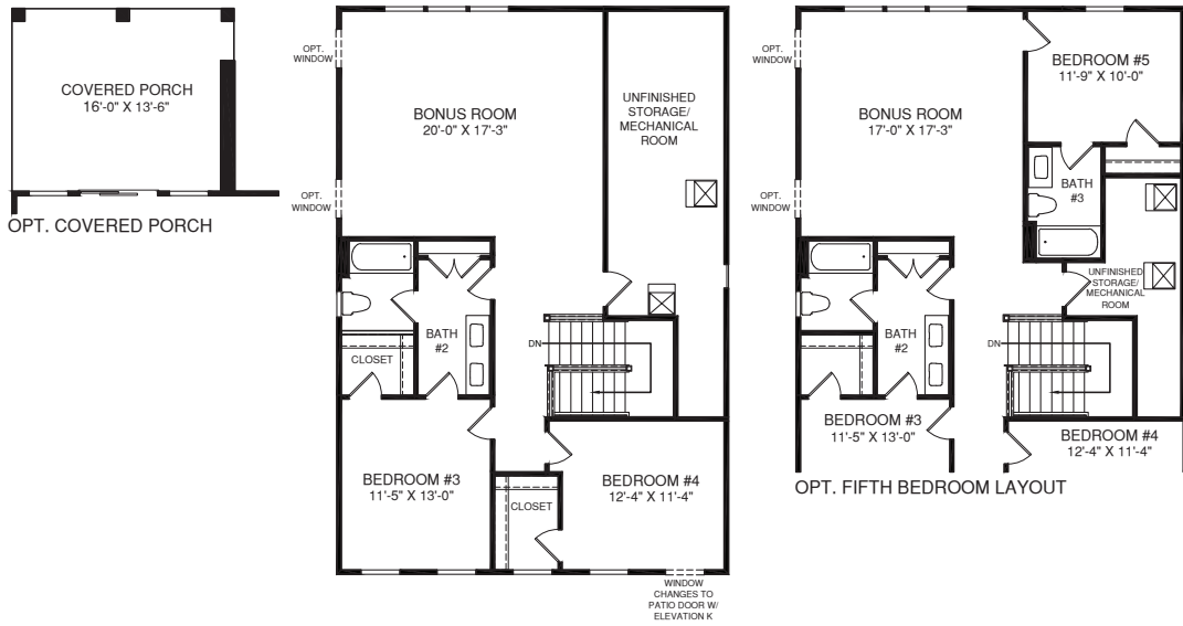
UPPER LEVEL
