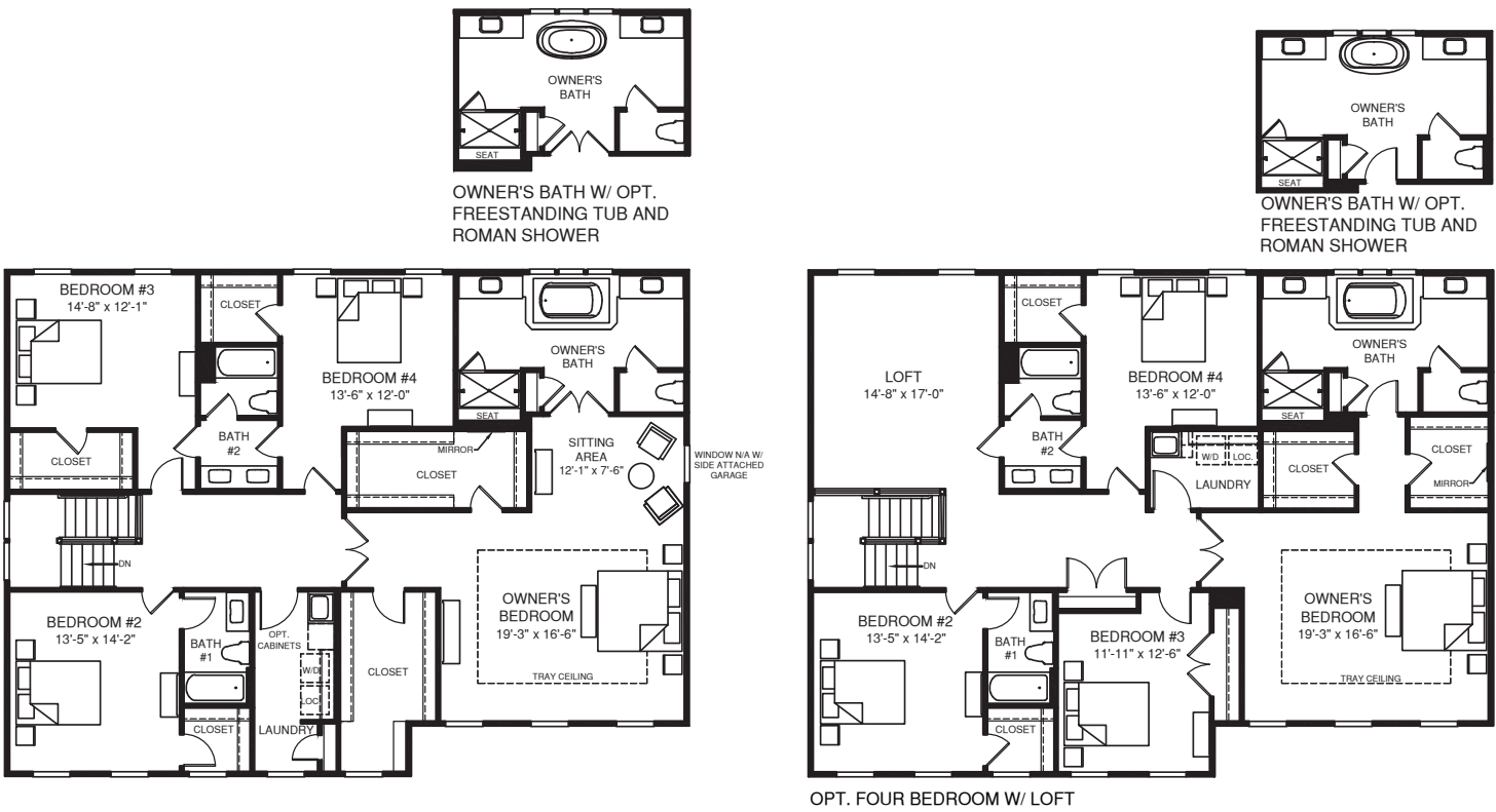
UPPER LEVEL
