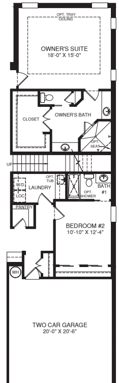
FLOOR PLAN W/ OPT. BONUS ROOM
