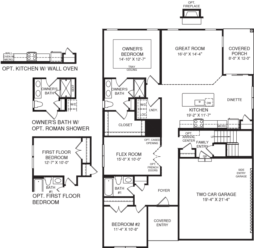
MAIN LEVEL
