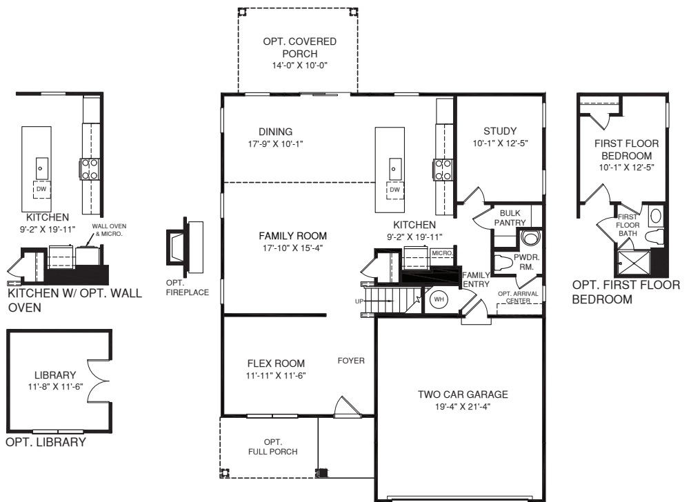
MAIN LEVEL
