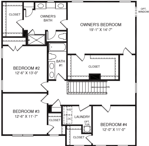
UPPER LEVEL
