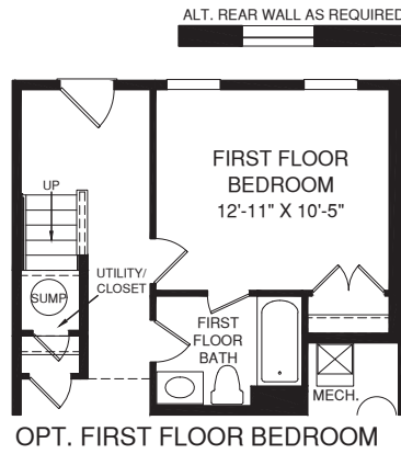
MAIN LEVEL
