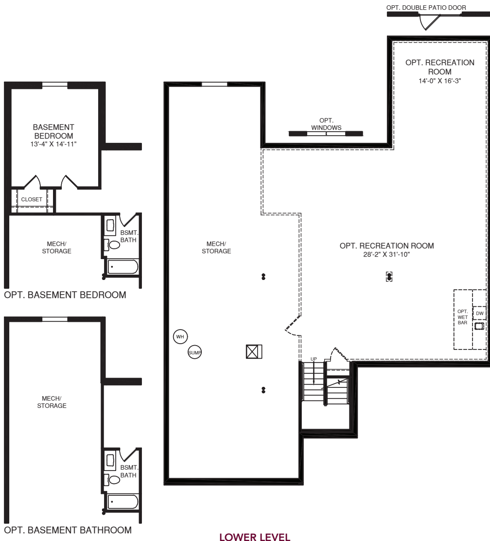
LOWER LEVEL
