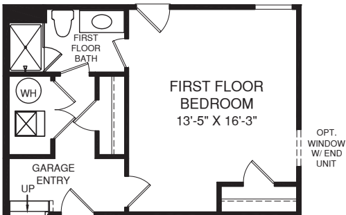
OPT. FIRST FLOOR BEDROOM
