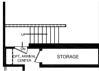
STAIRS W/ OPT. STEP-UP GARAGE
