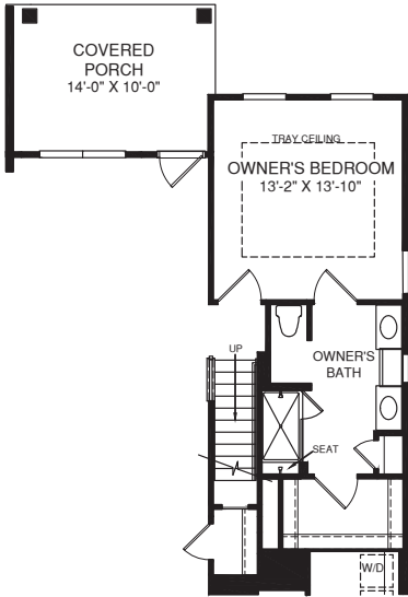
OPT. LUXURY OWNER'S SUITE SHOWN W/ OPT. COVERED PORCH
