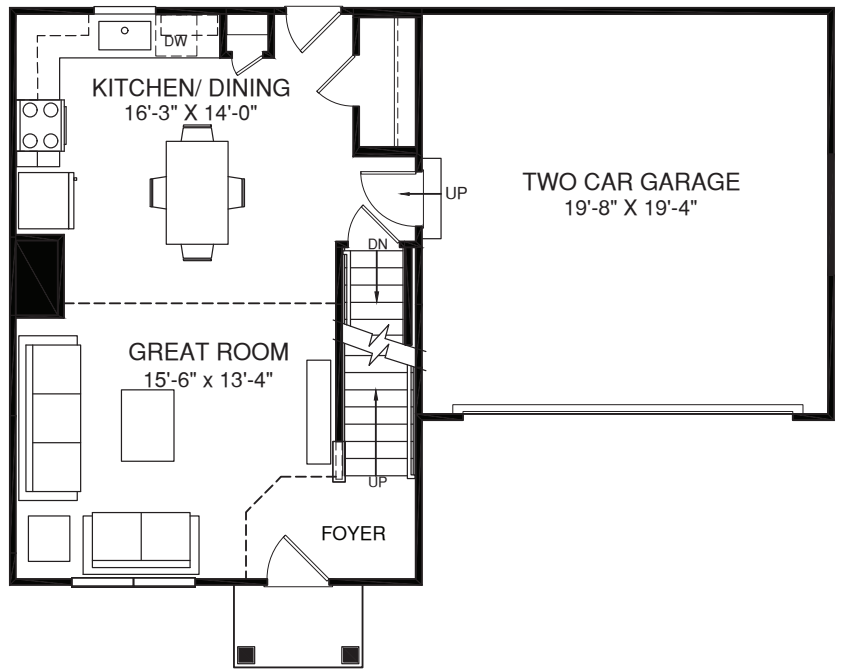
MAIN LEVEL
