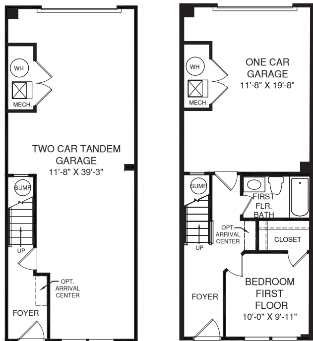
TWO CAR TANDEM GARAGE
