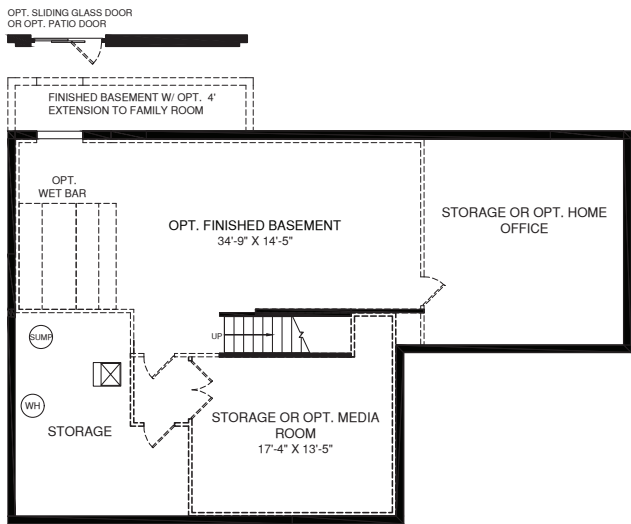
LOWER LEVEL
