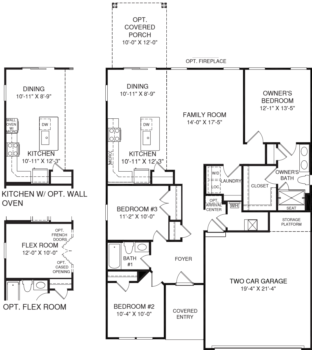
MAIN LEVEL
