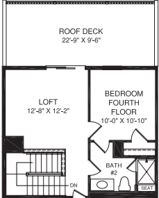
OPT. BEDROOM FOURTH FLOOR W/ OPT. 4'-0" EXTENSION TO HOUSE
