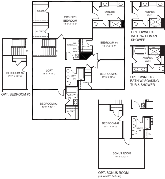
UPPER LEVEL
