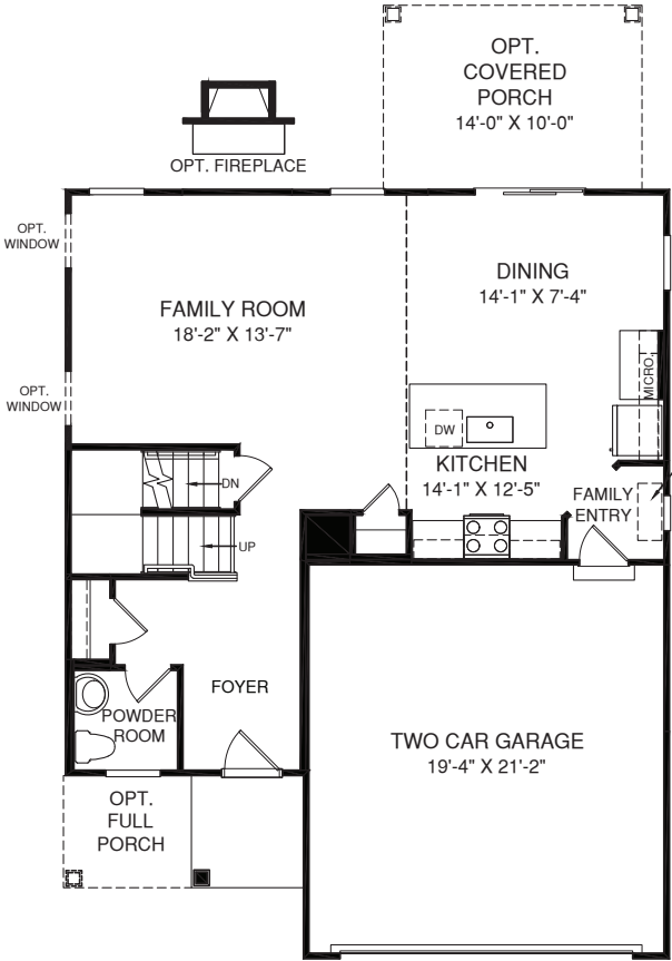
MAIN LEVEL
