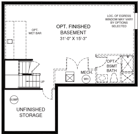
LOWER LEVEL
