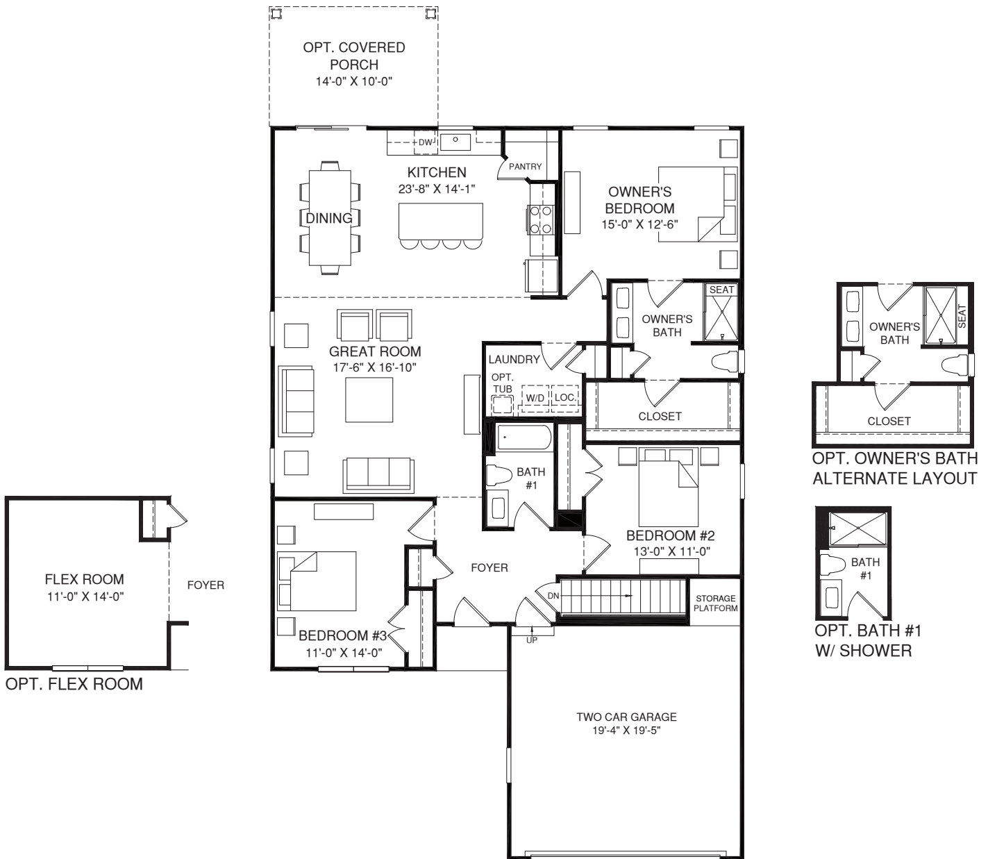
MAIN LEVEL
