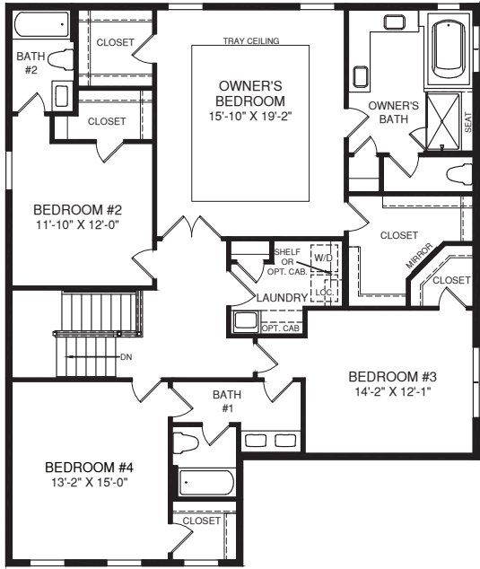
UPPER LEVEL
