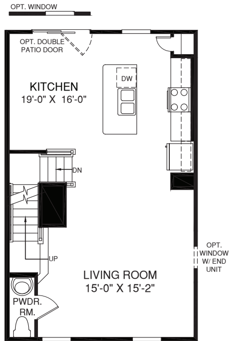
MAIN LEVEL
