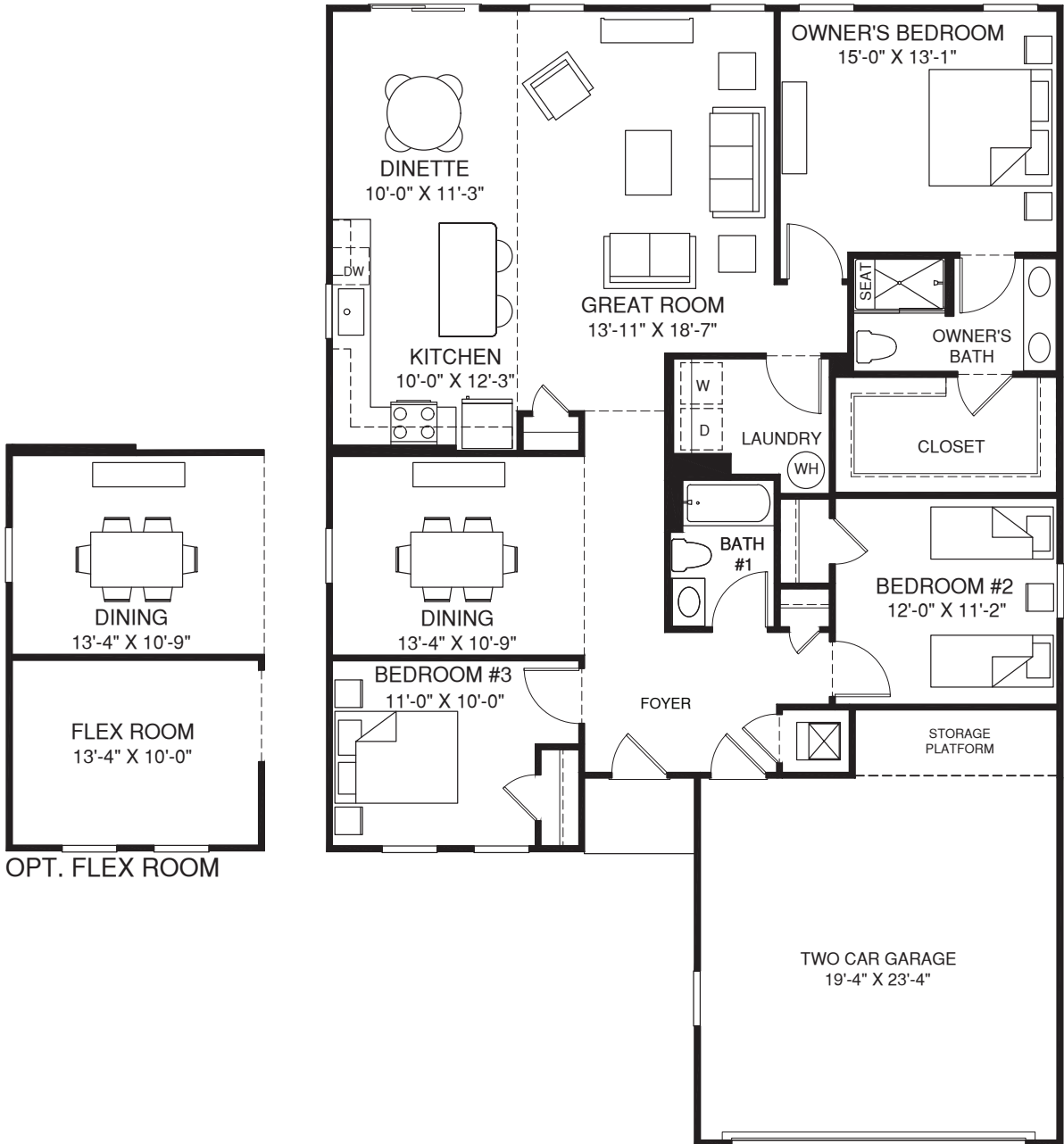
MAIN LEVEL
