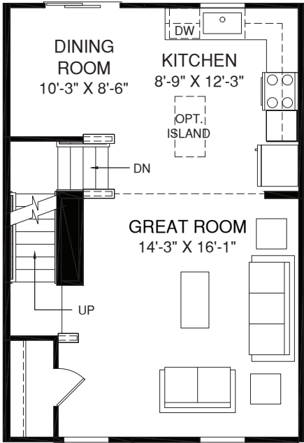
MAIN LEVEL
