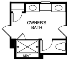
OPT. OWNER'S BATH W/ ROMAN SHOWER
