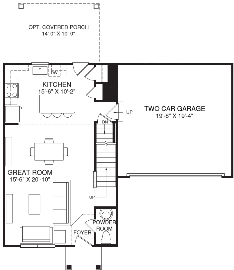
MAIN LEVEL
