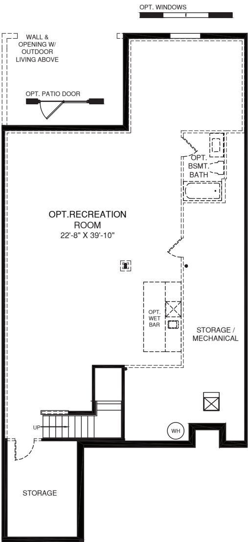
LOWER LEVEL
