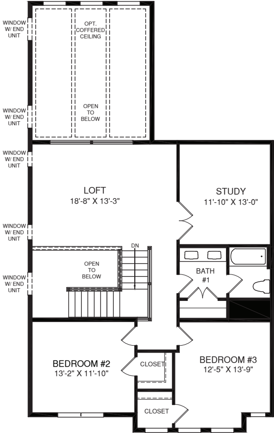
UPPER LEVEL
