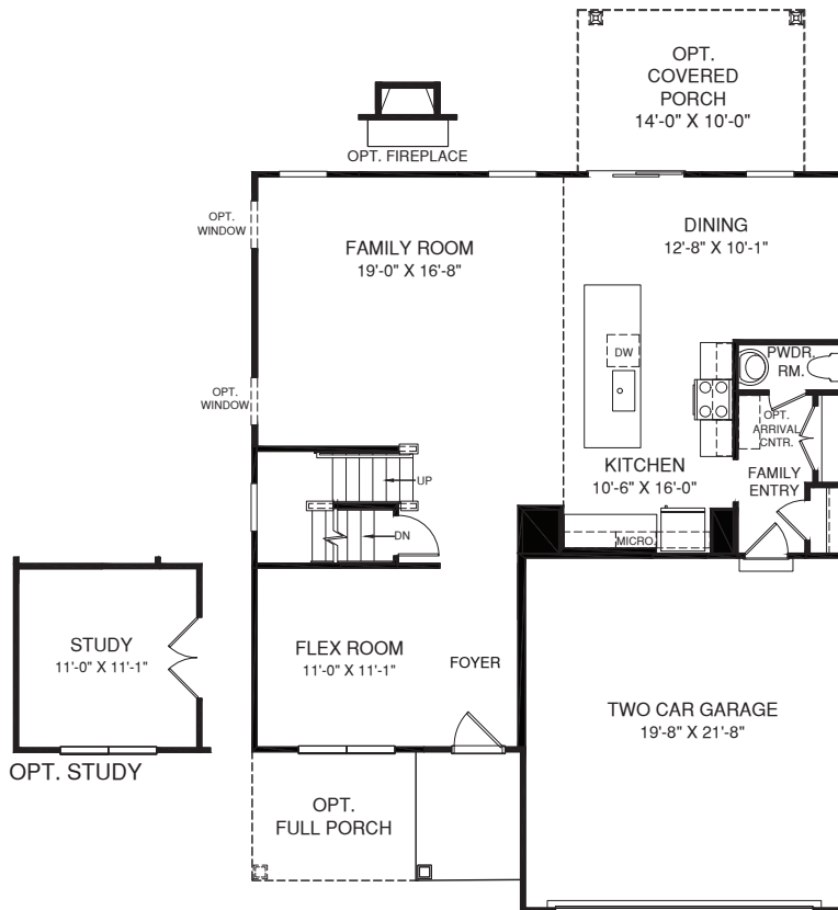
MAIN LEVEL
