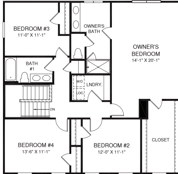
UPPER LEVEL
