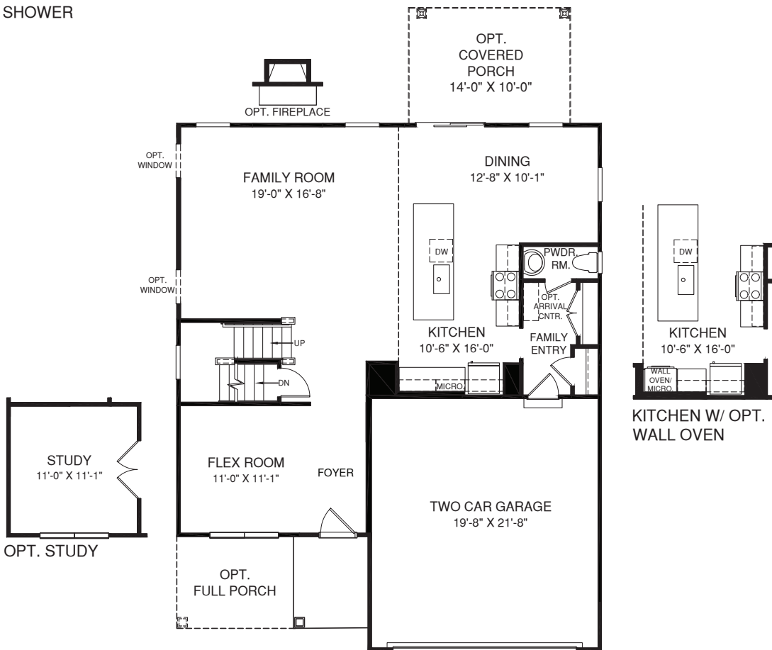
MAIN LEVEL
