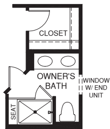
OPT. OWNER'S BATH SHOWER ALT. LAYOUT
