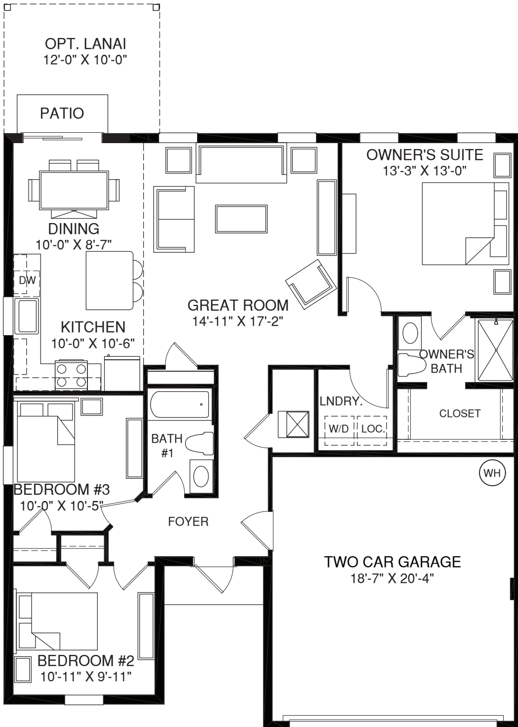
MAIN LEVEL
