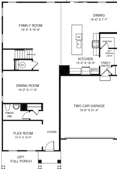
MAIN LEVEL
