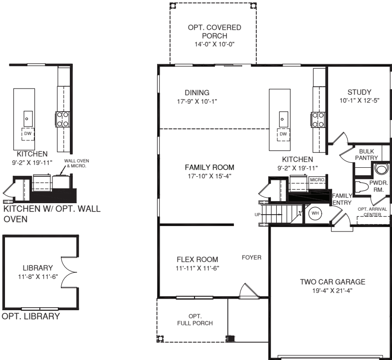
MAIN LEVEL
