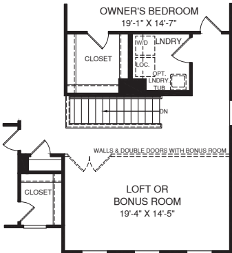
OPT. LOFT OR OPT. BONUS ROOM
