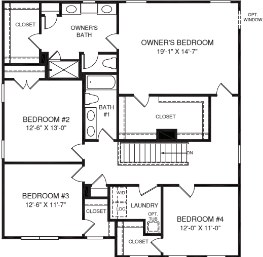
OPT. OWNER'S BATH W/ SOAKING TUB & SHOWER
