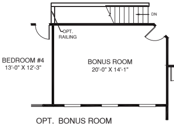
OPT. BONUS ROOM
