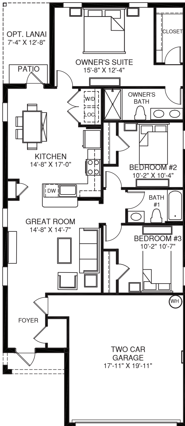
MAIN LEVEL
