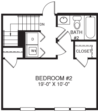
OPT. BEDROOM #2
