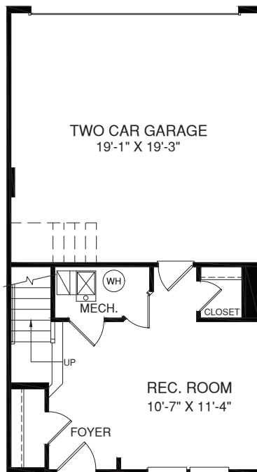
LOWER LEVEL
