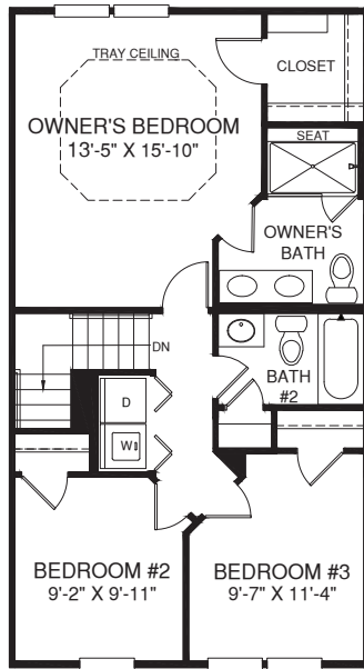
UPPER LEVEL
