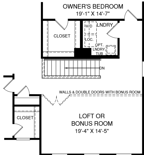
OPT. LOFT OR OPT. BONUS ROOM
