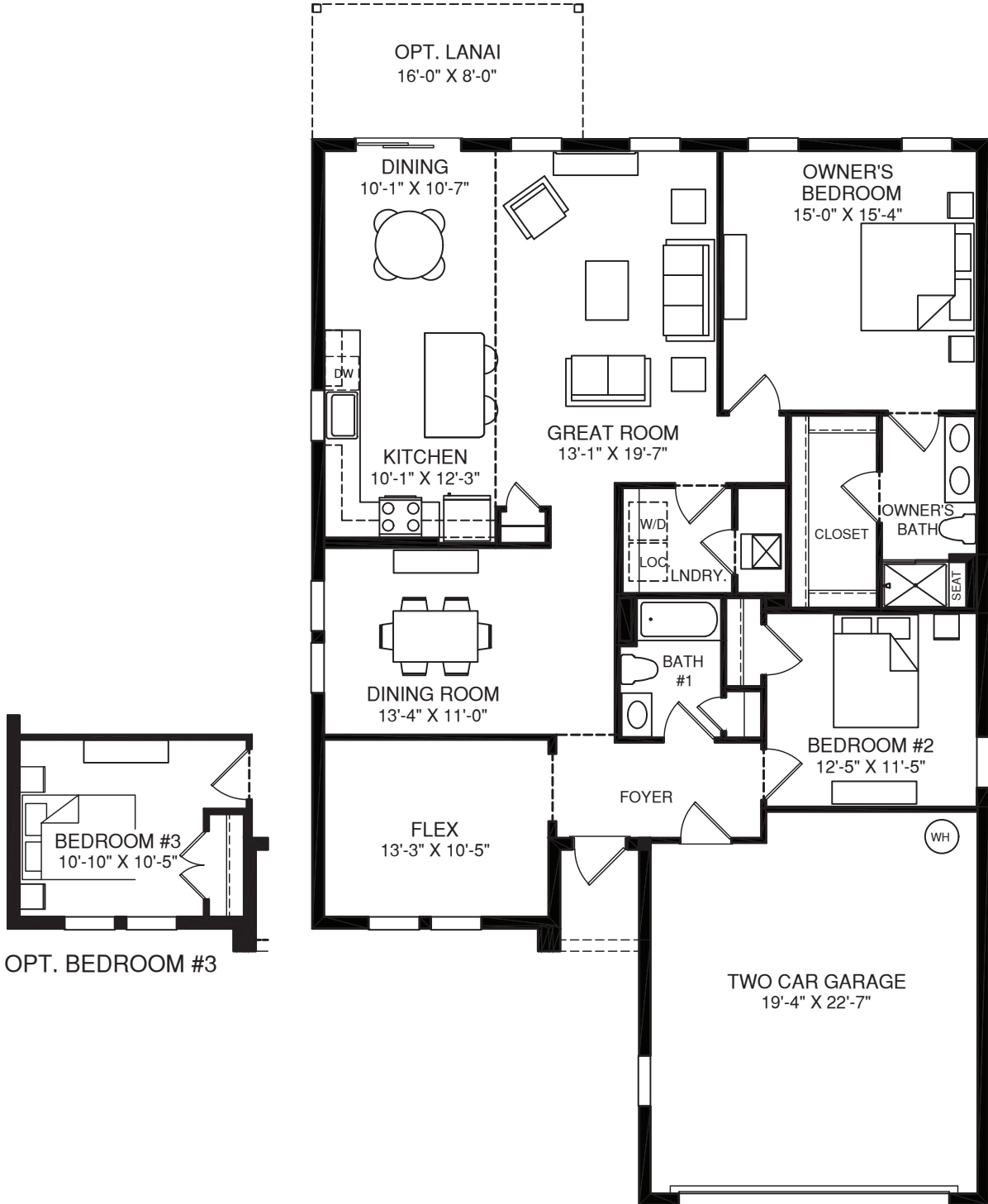
MAIN LEVEL
